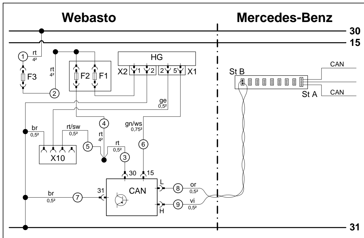
Wiring diagram
