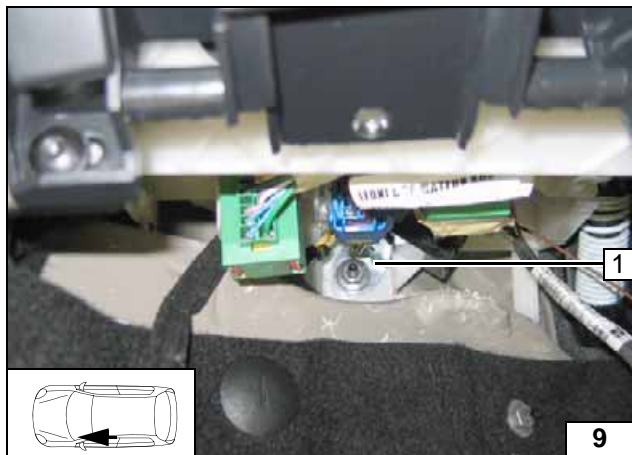
1 Angle bracket, original vehicle stud bolt, flanged nut
