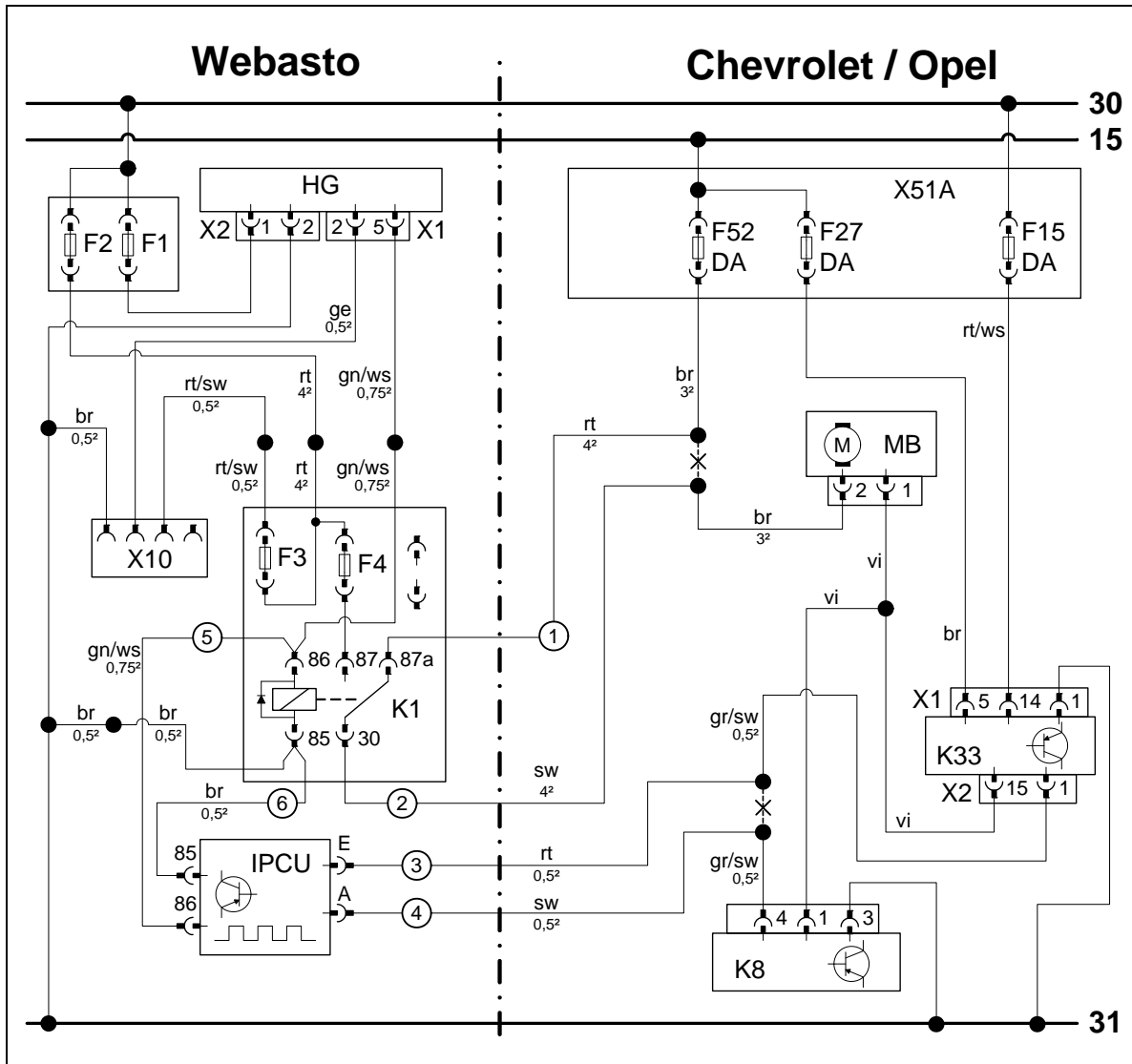
Wiring diagram
