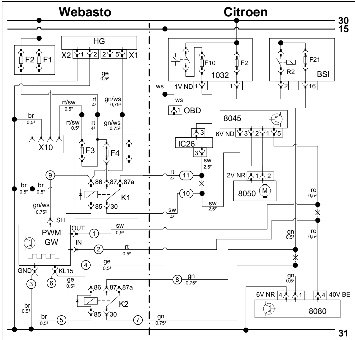
Wiring diagram
