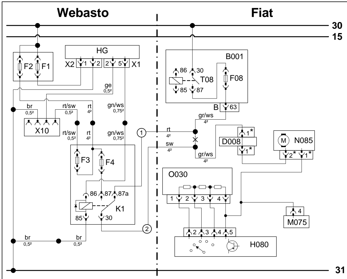
Wiring diagram
