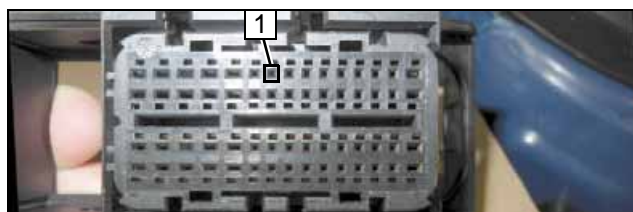
1 Pin 7 / engine control unit connector G, contact side
