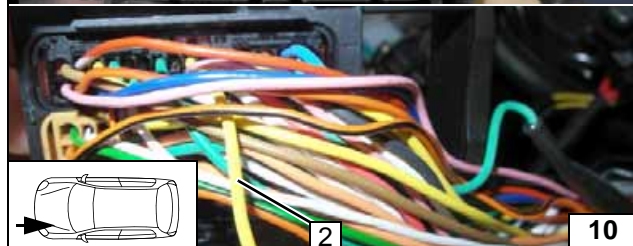
2 Yellow (ge) wire of engine control unit connector G pin 7, wiring side
