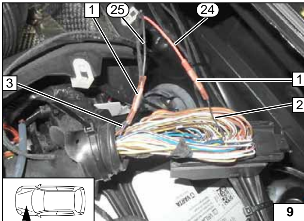
1 Crimp and shrink butt connector [2x] 2 Black/purple (sw/li) wire from connector B of MSG/ pin 33 3 Black/purple (sw/li) wire 24 Red (rt) wire of CLR module/ W wiring harness of cold start 25 Black (sw) wire of CLR module/ A wiring harness of cold start
