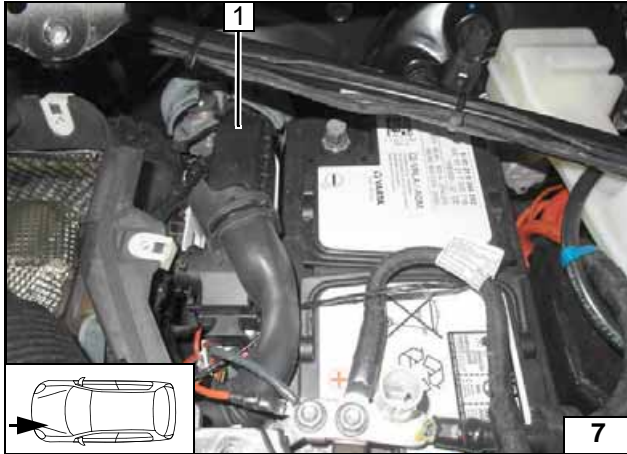
1 96-pin connector of MSG
