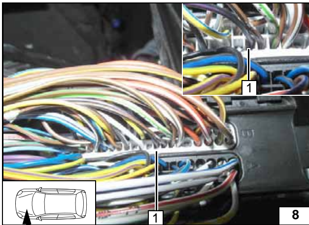
1 Black/purple (sw/li) wire from connector B of engine control unit, pin 33
