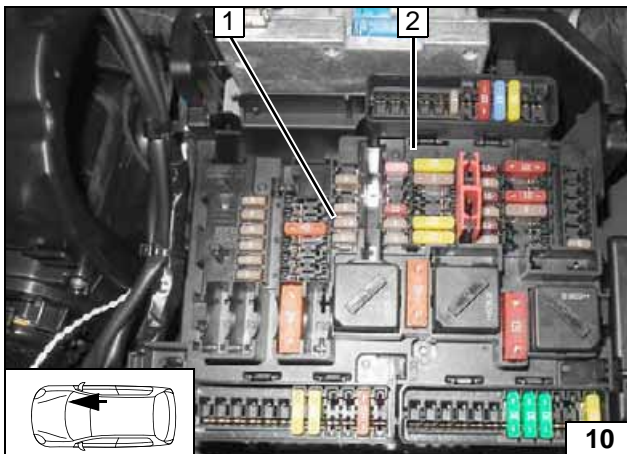
1 Position of F53 fuse 2 Passenger compartment fuse and relay box
